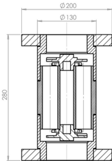
Raccord: 3"
